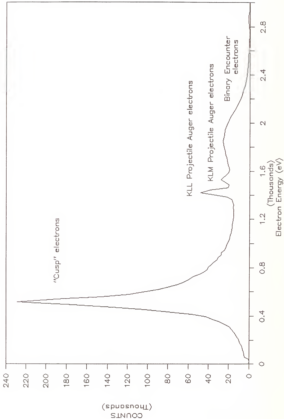
Figure 1. Electron emission spectra taken at 0^0 with respect to the beam axis involving 0.92 MeV/u C^{+3} projectiles incident on He gas
